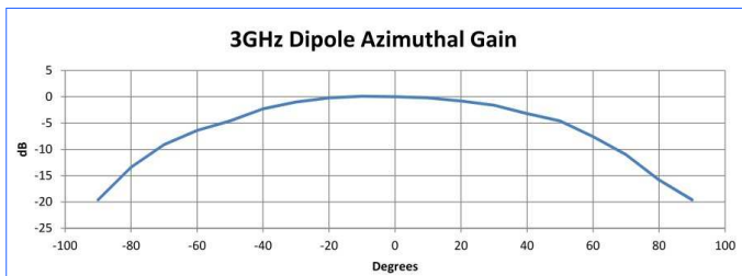
Azimuth Gain at 3GHz
