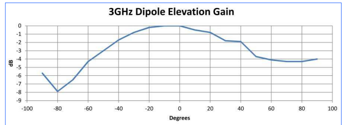
Elevation Gain at 3GHz
