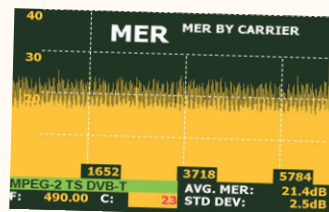
Echo effect out of the Guard Interval (40 μs). The ripple is observed in the graphic and the average of MER has significantly lessened.
