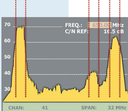
We can confirm that this is the source of the problem just by comparing the graphic with the spectrum analyser display of an analogue channel
