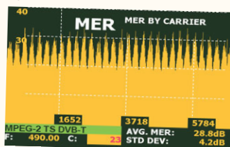
Echo effect inside the Guard Interval (4 μs). The ripple is observed in the graph, but the average of MER is not practically affected.
