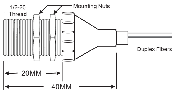
Sensor Head
