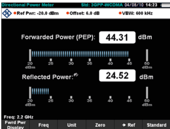
Measurement of the forward (TX output) and the reflected power of an antenna.
