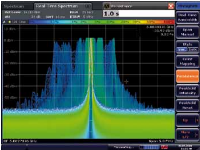
Transient response of a VCO for WLAN applications in persistence mode.
