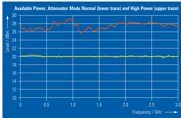
Typical maximum output power versus frequency (with and without high-power output option)
