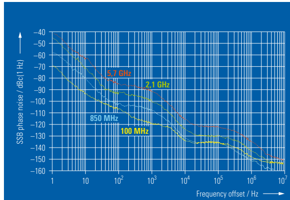
Typical SSB phase noise at 100 MHz, 850 MHz, 2.1 GHz and 5.7 GHz with internal reference oscillator (without low phase noise option)
