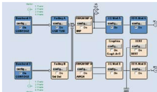
Generation of a GSM/EDGE frame with faded and unfaded timeslots
