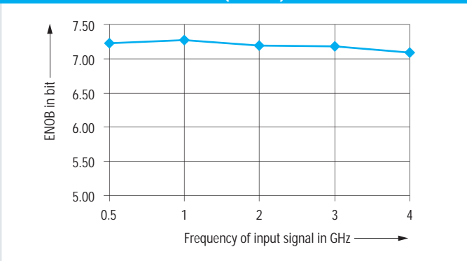
Effective number of bits (ENOB)
