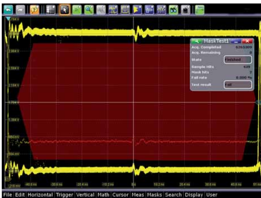
High-speed mask test with R&S®RTO oscilloscopes: Within ten seconds, more than six million waveforms are acquired, evaluated and displayed.
