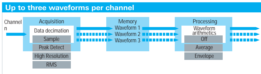
The R&S®RTO oscilloscopes are the first to allow users to configure the type of data decimation and the waveform arithmetics and to display up to three waveforms simultaneously.
