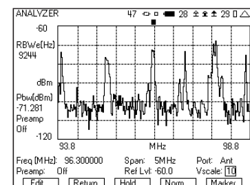
Spectrum Analyzer monitoring over the air showing multiple transmitters
