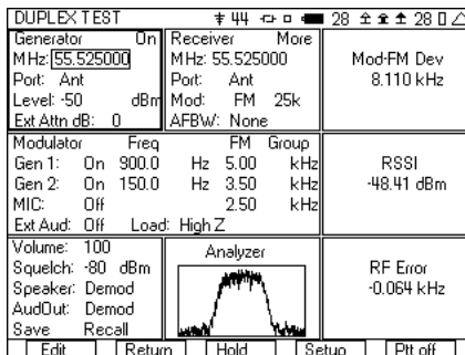
Duplex Screen showing VHF FM radio test
