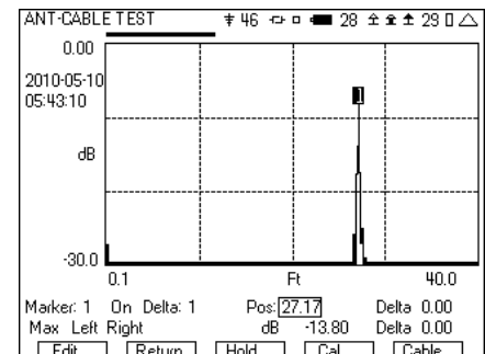
Ant-Cable Test showing a distance measurement of a 27 foot coax
