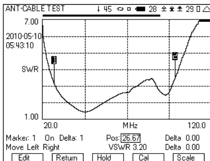
Ant-Cable Test showing a VSWR sweep of a 30 to 90 MHz antenna
