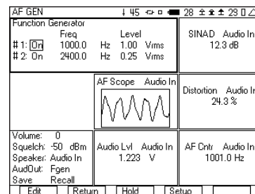
Audio Test showing a typical stimulus and response of an audio intercom
