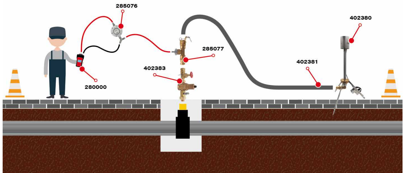
Connection example with the Mobile Gas Flare M
