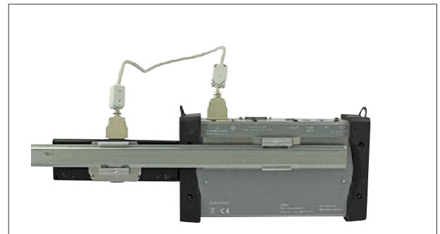
Montage Rail Din Reference : 902403000 for DAS240 (up to 60 channels) Reference : 902201000 for DAS220
