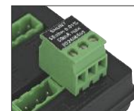
50-ohm shunt (4-20mA) for DAS220 and DAS240 Reference: 902406500
