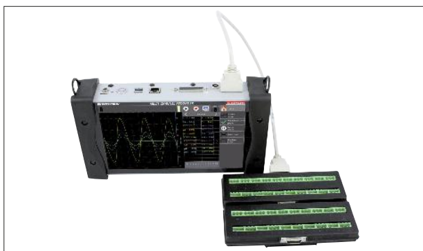
DAS240 equipped with 40 measurement channels
